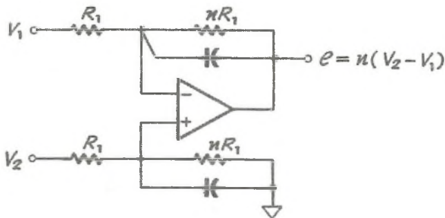
Adder-Subtractor
