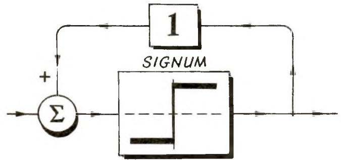
Figure 9. Hysteresis Element
