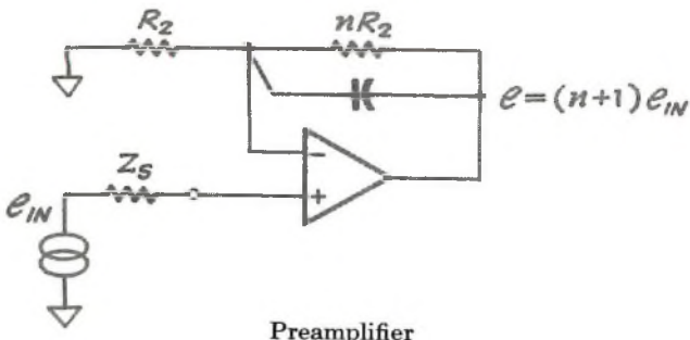
Preamplifier
