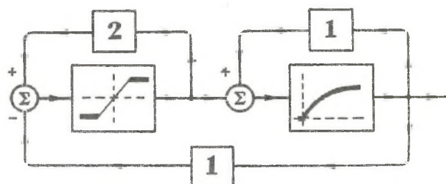
Figure 15. Typical (+/-) Feedback System
