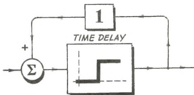
Figure 13. Staircase Integrator
