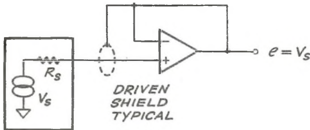
Unity Gain Follower
