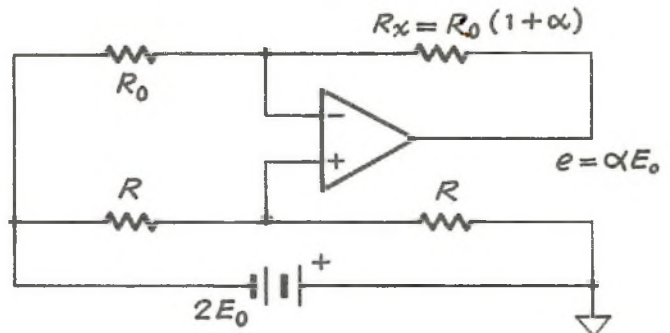
Bridge Amplifier
