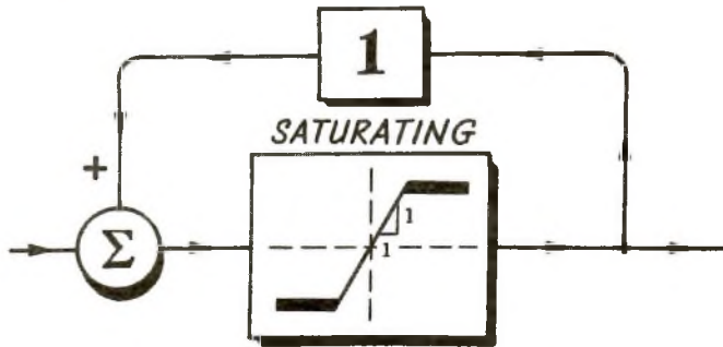
Figure 7. Signum Element
