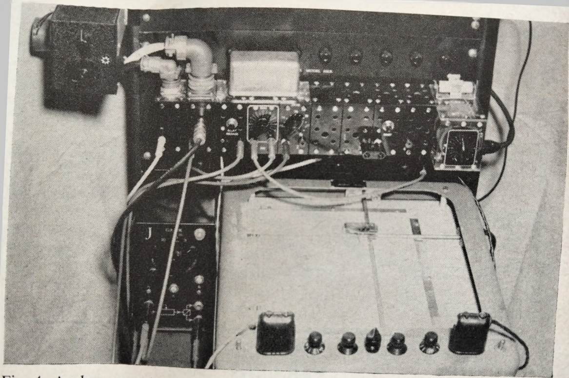
Fig. 4. Analog computer and x-y plotter. Calibrator is shown on the extreme upper left. The K3J integrator (George A. Philbrick Researches, Inc.) is to the left of the x-y plotter.
